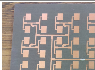
Microstrip array antenna for X-band radar
